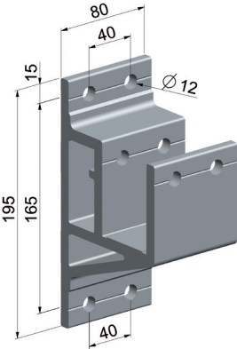
Soporte frontal/techo Wall/ceiling support
